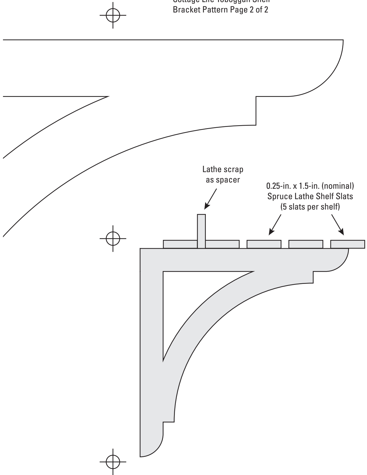
Bracket layout on 1x8x5' pine board
