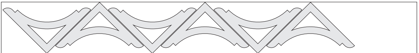
Bracket layout on 1x8x5' pine board
